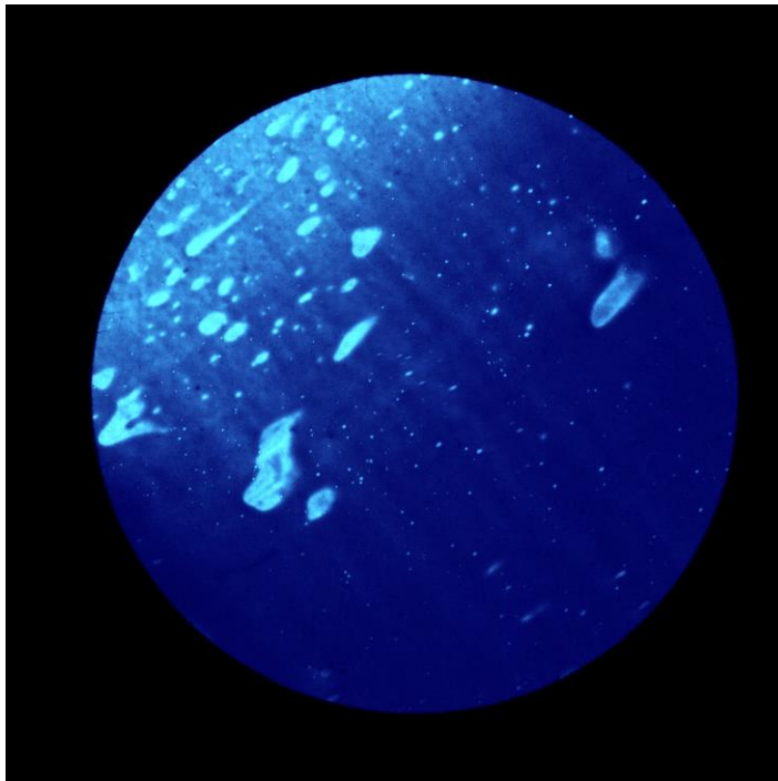
BSO N815 (blue stellar objet), 2001. Cortesía Aleydis Rispa
